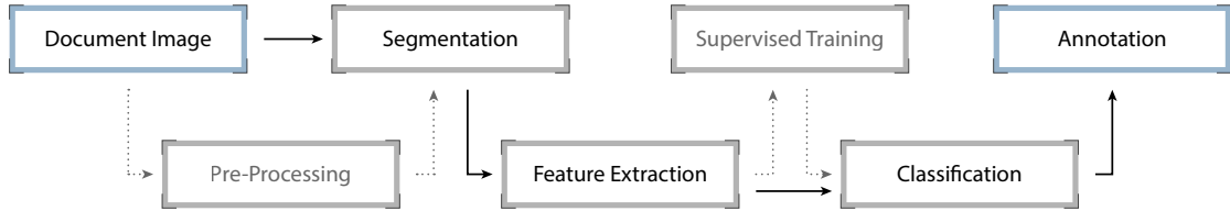
Figure 2.13: Design of a basic text classification system.
