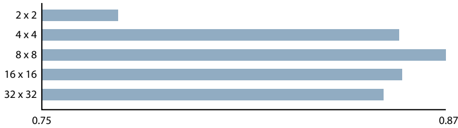
Figure 4.30: Varying the feature dimension between 4 and 1024. A 8 \times 8 log polar grid is best suited for the text classification.
