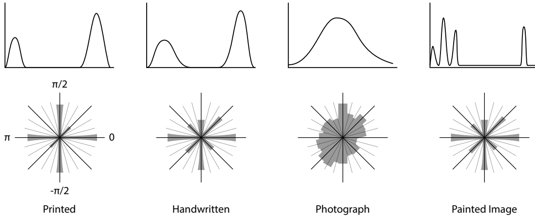
Figure 2.6: Schematic illustration of the Imaged features. The upper row shows the luminance features for all four classes respectively while the lower line illustrates the gradient features.
