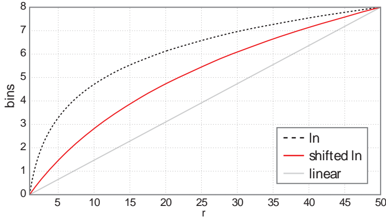
Figure 4.11: Logarithmic bin sampling. The ordinate shows the feature’s bins while the abscissa shows the Cartesian coordinates in the spatial domain. Note that the first 5 pixel are accumulated to 3 bins if ln is applied.
