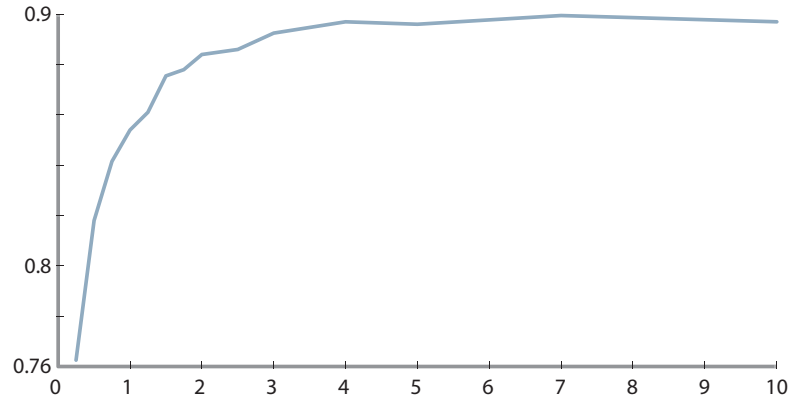
Figure 4.31: Precision if the feature's scale factor s is varied between 0.25 and 10.
