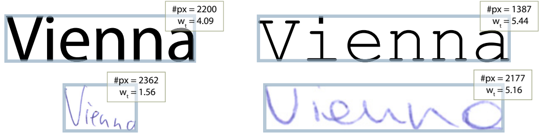
Figure 4.18: Two printed examples (upper row) and two handwritten examples (lower row) with the CC area per BB ( \#px ) and the BB ratio w_t proposed.
